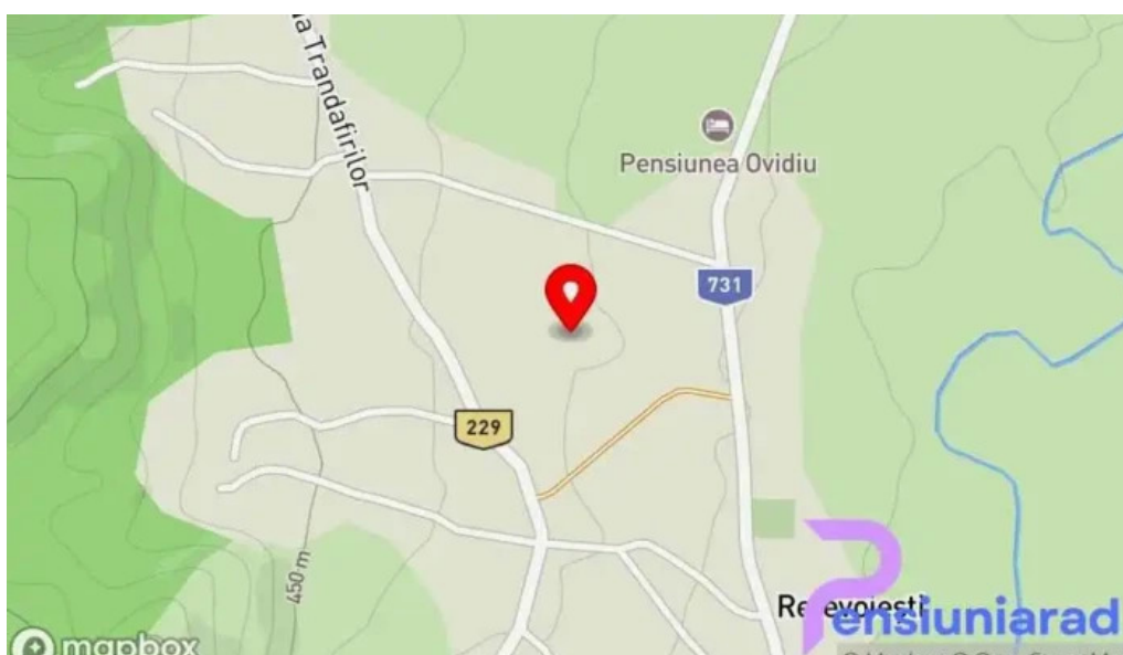
Retevoiesti hart?
